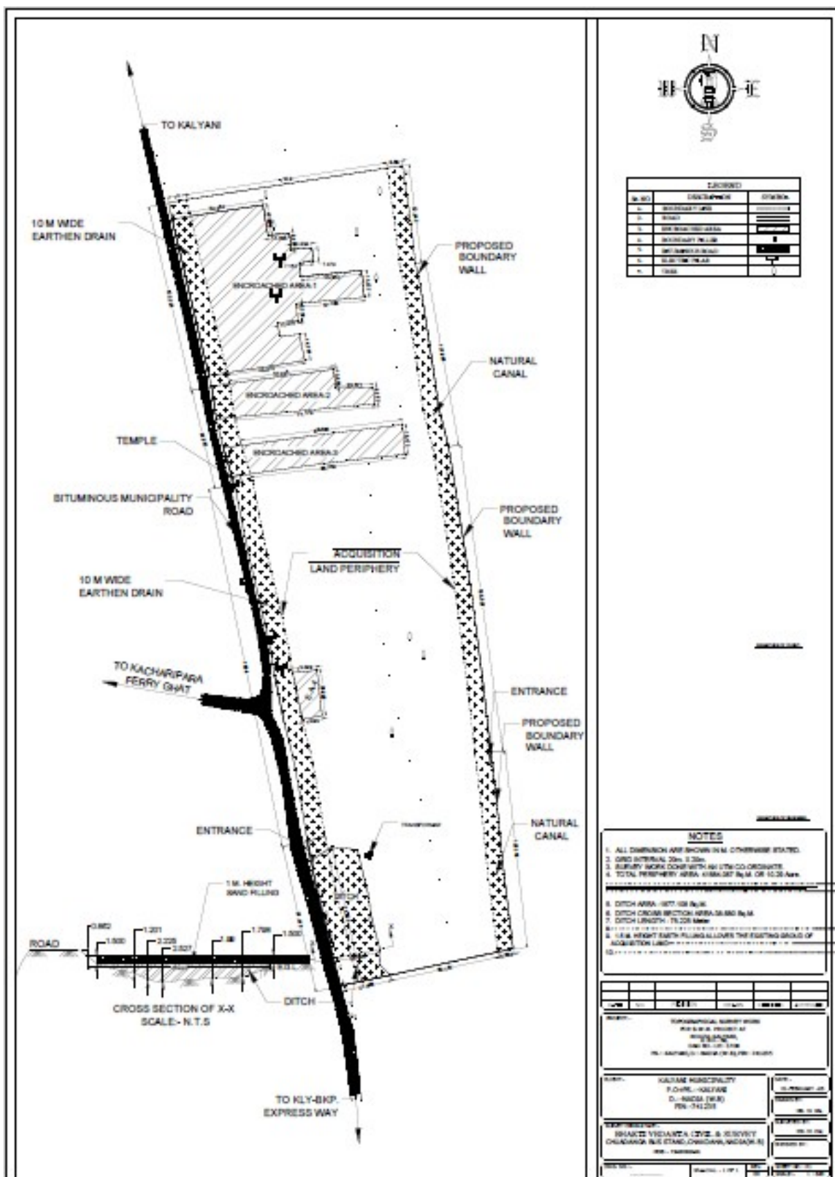
LINE DIAGRAM OF THE IDENTIFIED SITE AT MOUZA: KALYANI, P.S.: KALYANI, J.L. NO.: 58, L.R. PLOT NO.: 1708, WARD NO.: 8, KALYANI MUNICIPALITY [AREA: 10.274 ACRE]
